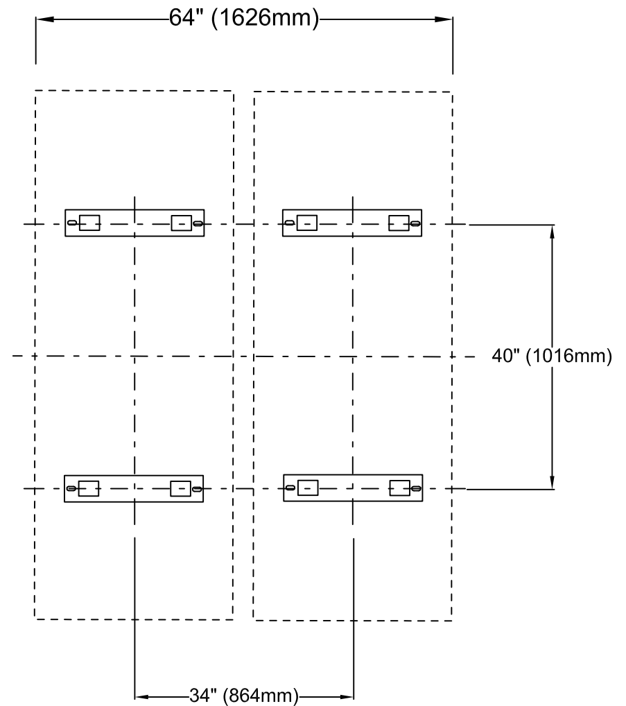
STORAGE CRADLE SPACING RECOMMENDATION FOR TON CONTAINER STORAGE
