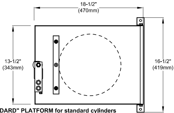
"STANDARD" PLATFORM for standard cylinders
