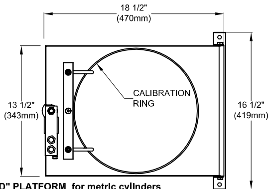
"SLOTTED" PLATFORM for metric cylinders
